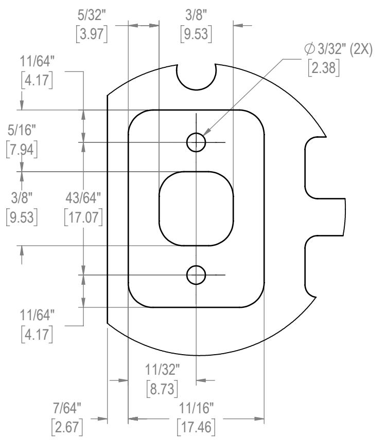
DETAIL D SCALE 2 : 1
